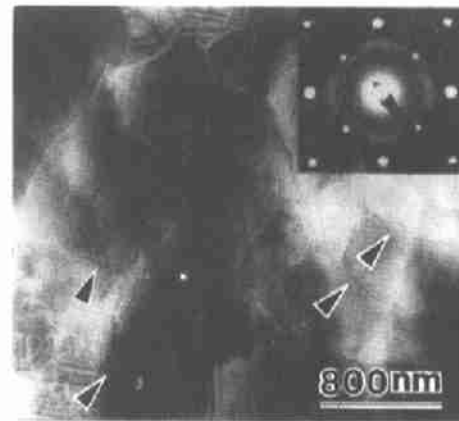
图 3 雾状单晶 (001) 晶片孪生畴的典型 TEM 像及选区电子衍射斑点 Fig.3 Typical TEM micrograph of the twin domains and the corresponding SAED pattern on (001) plate in translucent crystal
