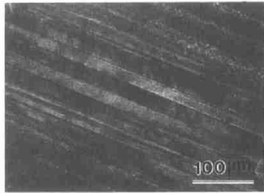
图 2 (001) 晶片正交偏光下的孪生畴 Fig.2 Twin domain under crossed polarized light on (001) plate
