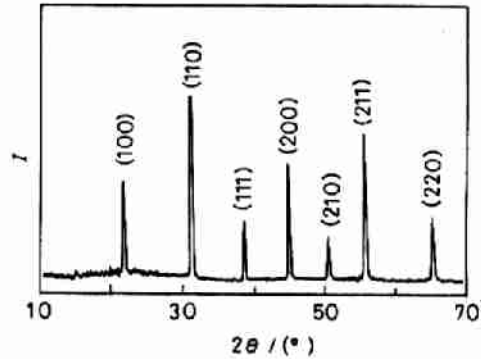
图 7 67PMN-33PT 单晶的粉末 X 射线衍射谱 Fig.7 XRD pattern of powder ground from single crystal
